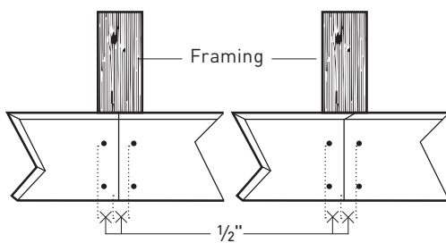
Butt Joint
