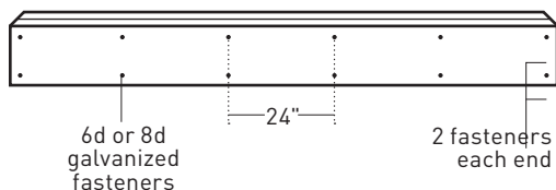
Double Nailed
