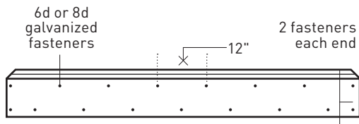
Stagger Nailed
