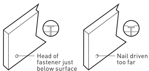
Surface Nailing
