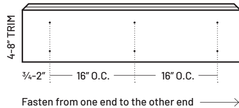
Double Nailed
