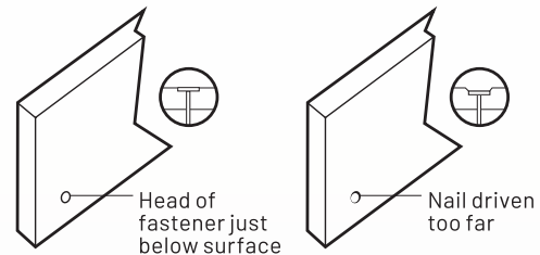
Surface Nailing
