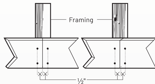
Butt Joint
